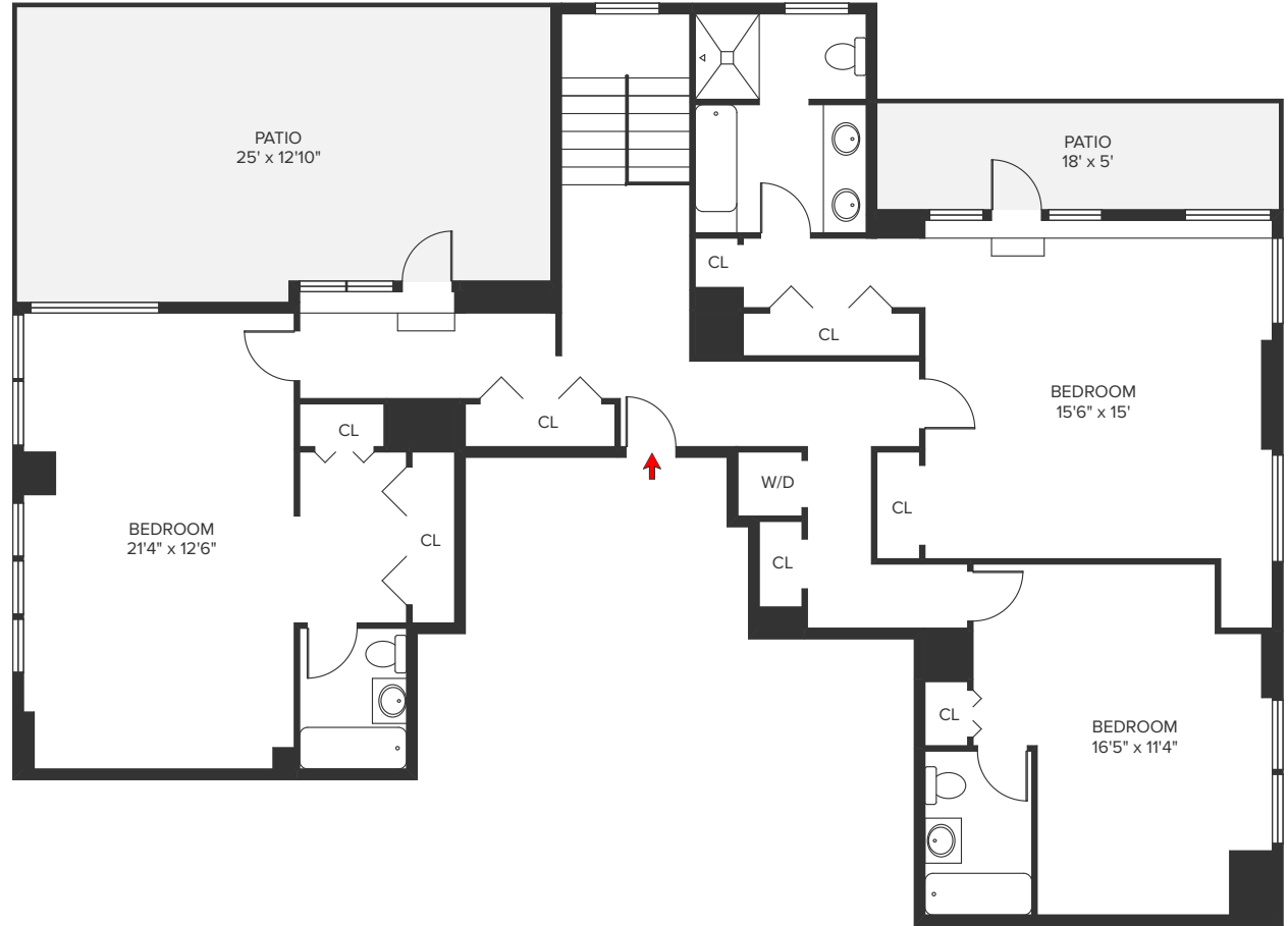
SECOND LEVEL
